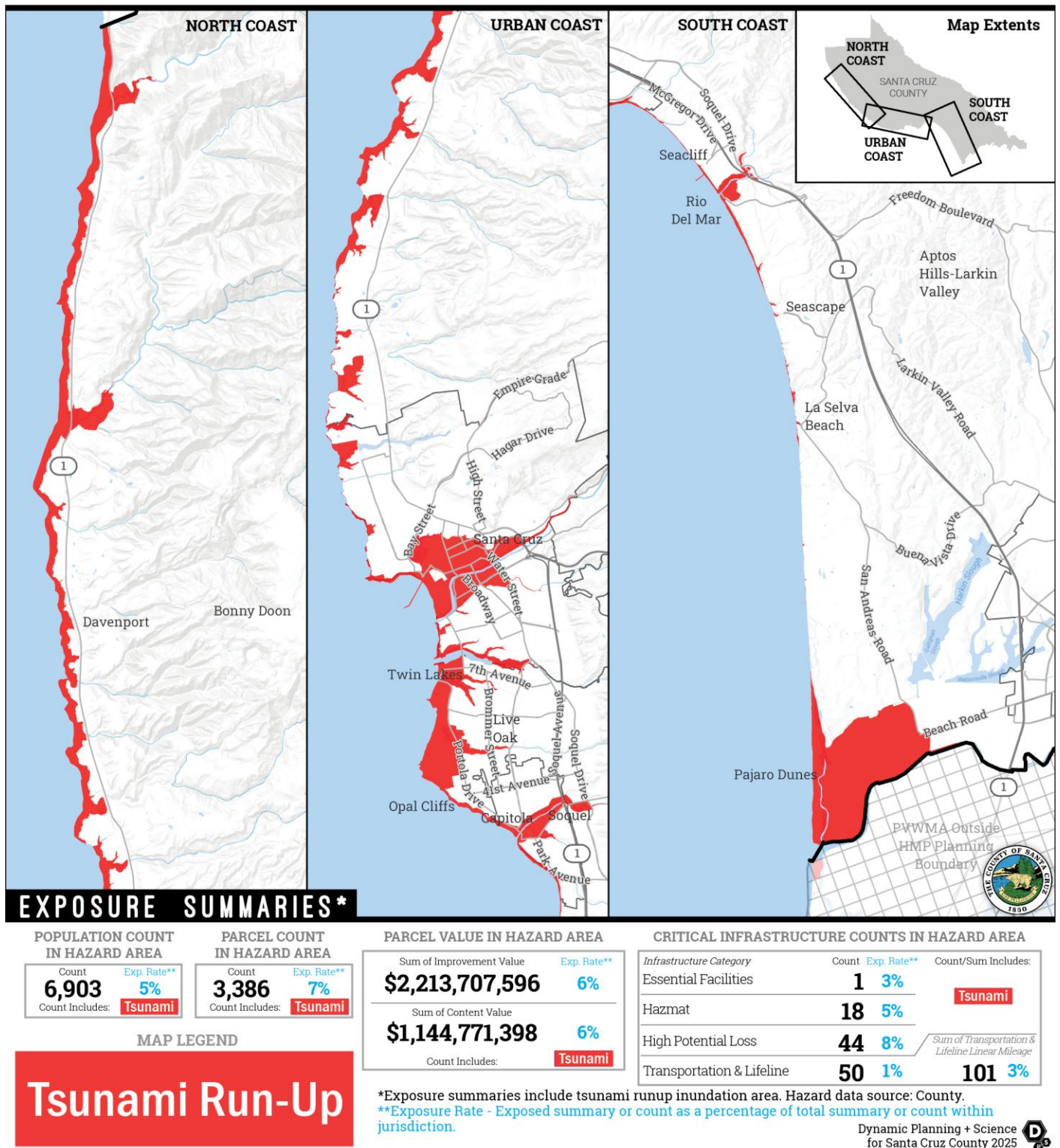
Figure 3-51: Exposure Summary - Santa Cruz County Tsunami Run-Up Areas
