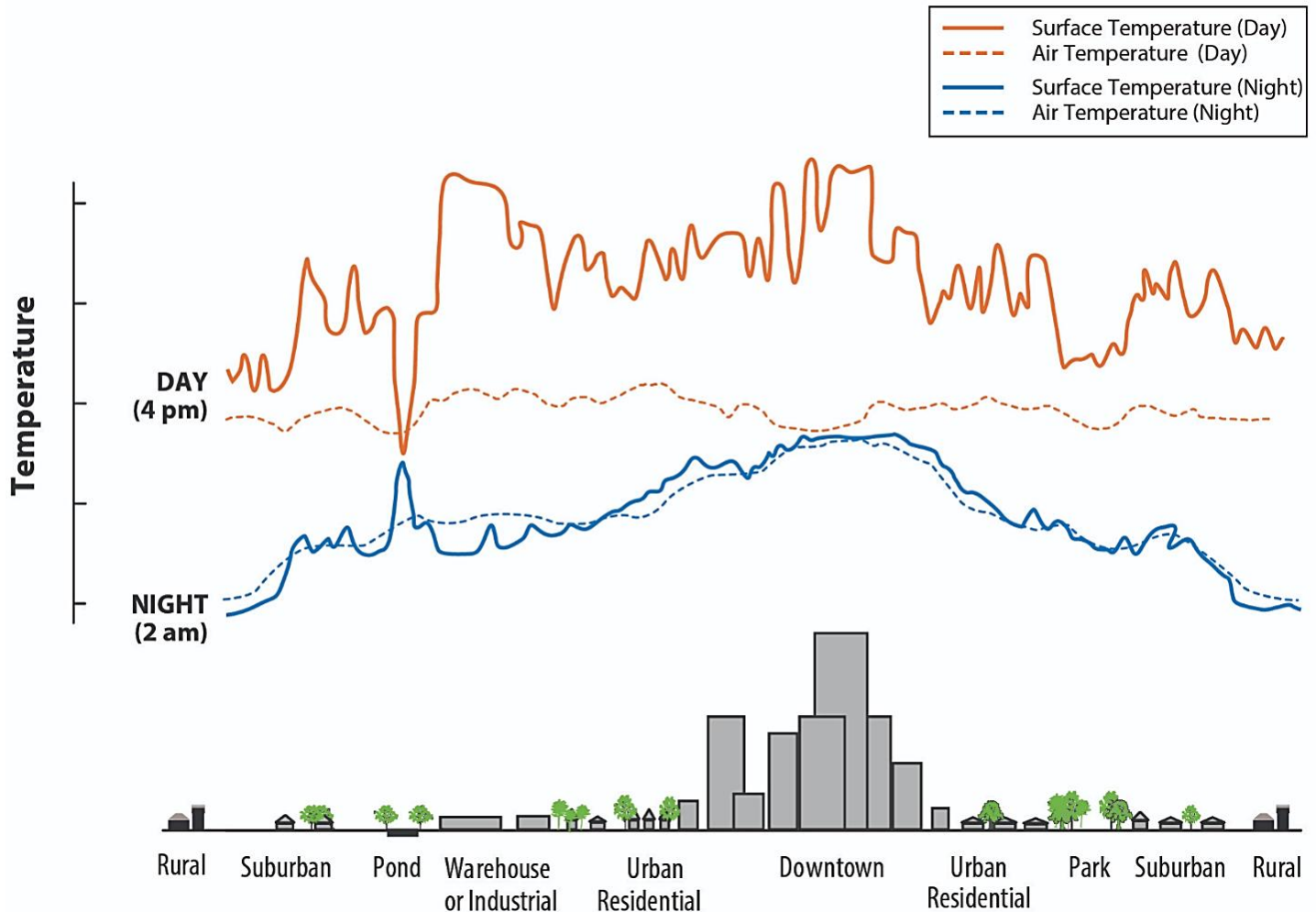
Figure 3-65: Day and Night Urban Heat Island Effect Across Natural and Built Landscapes
