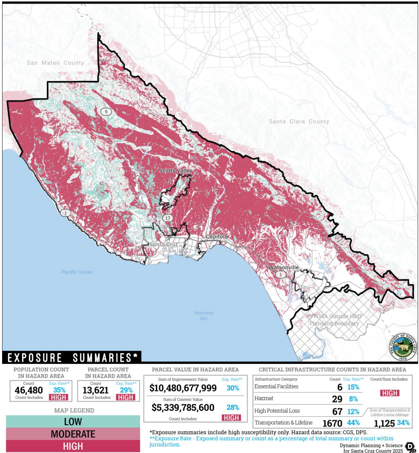
Figure 3-55: Exposure Summary - Santa Cruz County Slope Failure Risk
