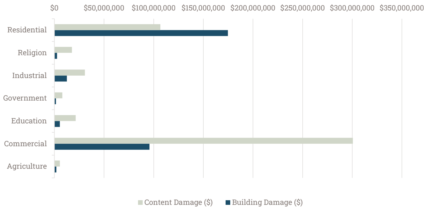
Figure 3-32: Santa Cruz County 100-YR Riverine Flood Damage Estimates by Building Type
