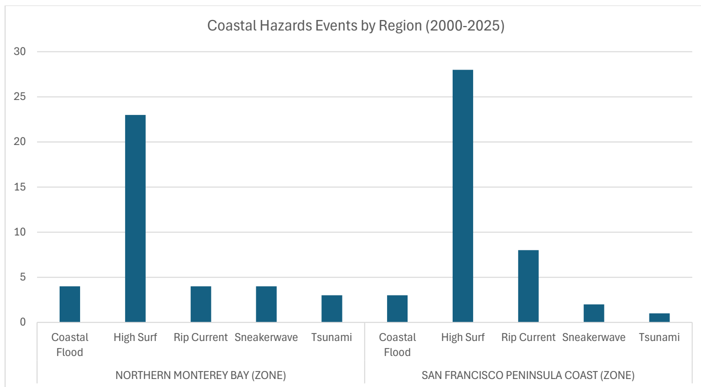
Figure 3-48: Santa Cruz County Coastal Hazard Events, 2000 -Present
