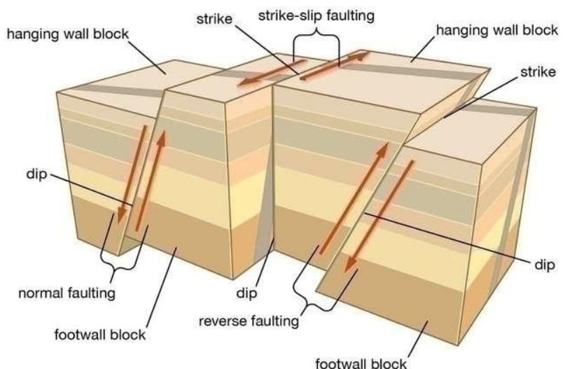
Figure 3-34: Earthquake Faulting
