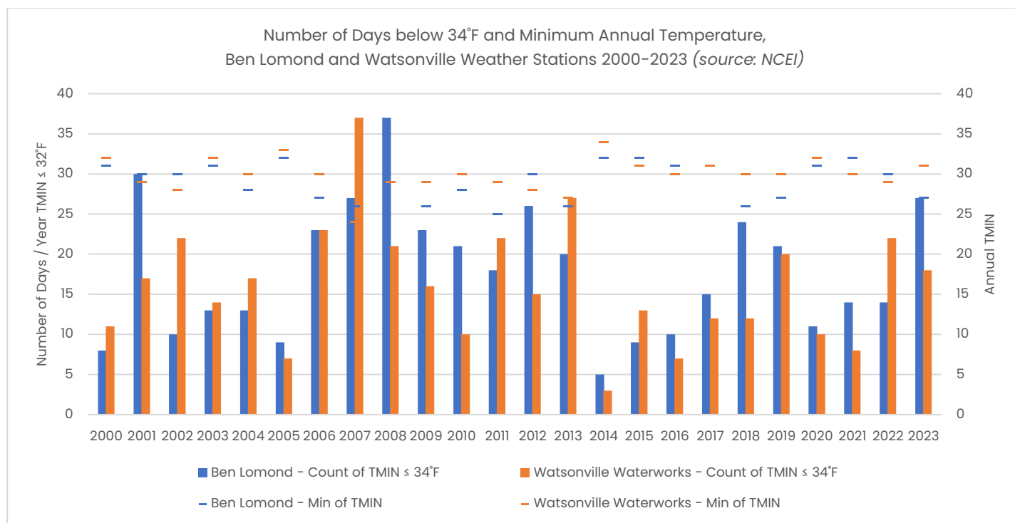
Figure 3-43: Minimum Annual Temperatures
