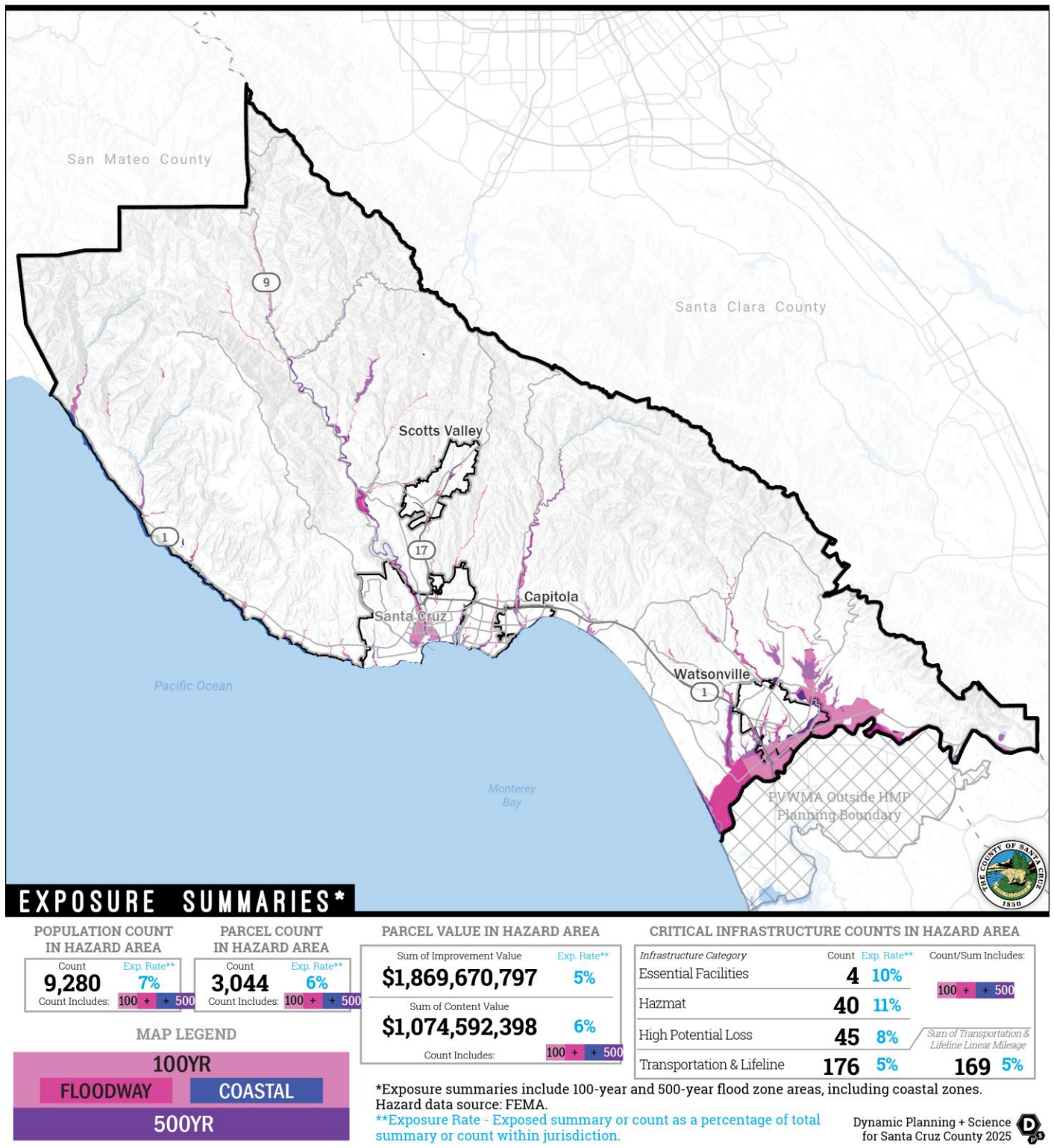
Figure 3-29: Exposure Summary – Santa Cruz County Flood Risk (FEMA Zones)
