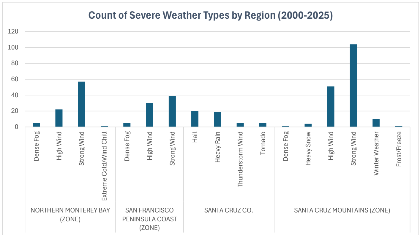
Figure 3-42: Severe Weather Events Recorded by NOAA
