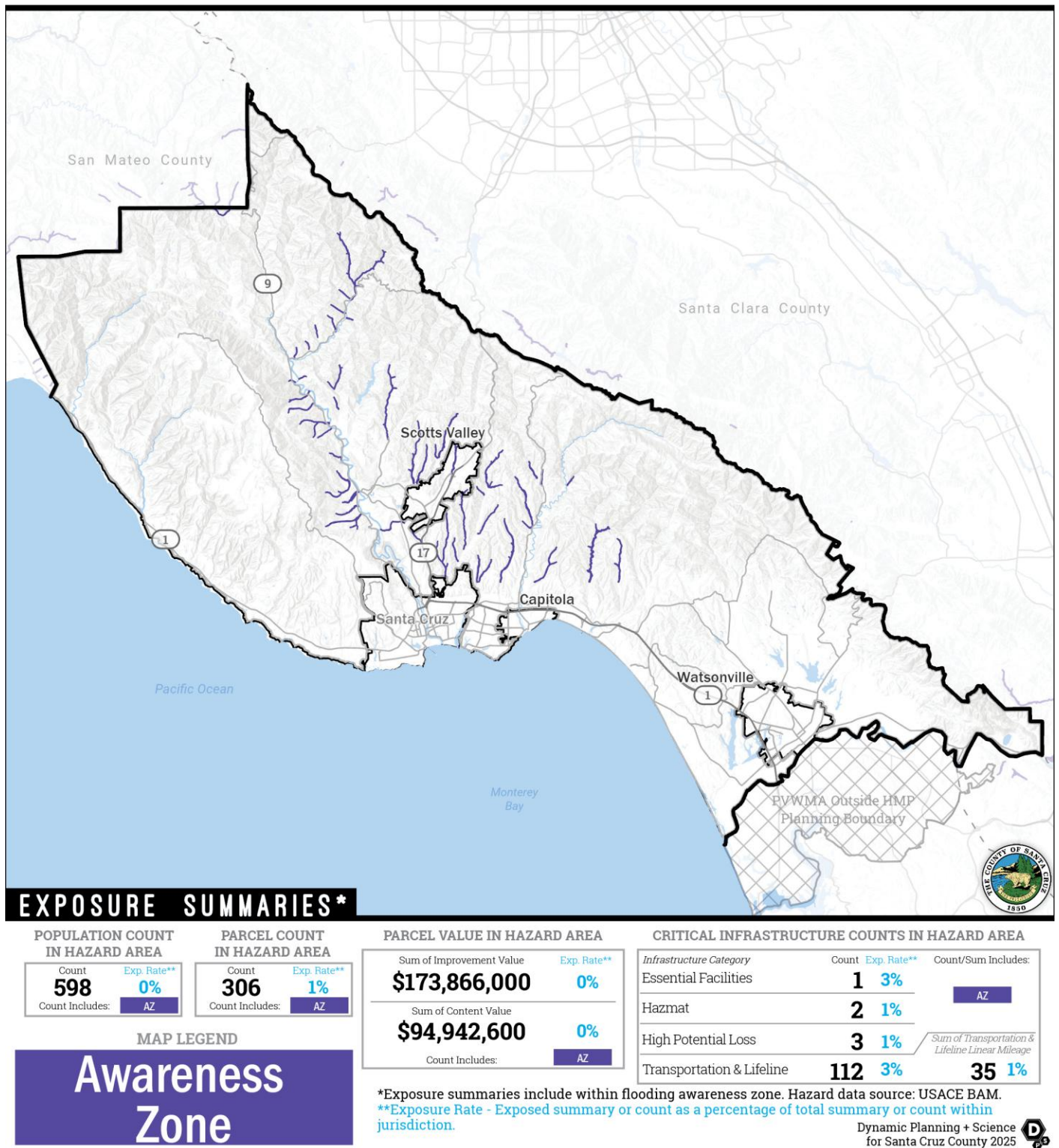
Figure 3-30 Exposure Summary – Santa Cruz County Flood Risk (DWR Awareness Zones)
