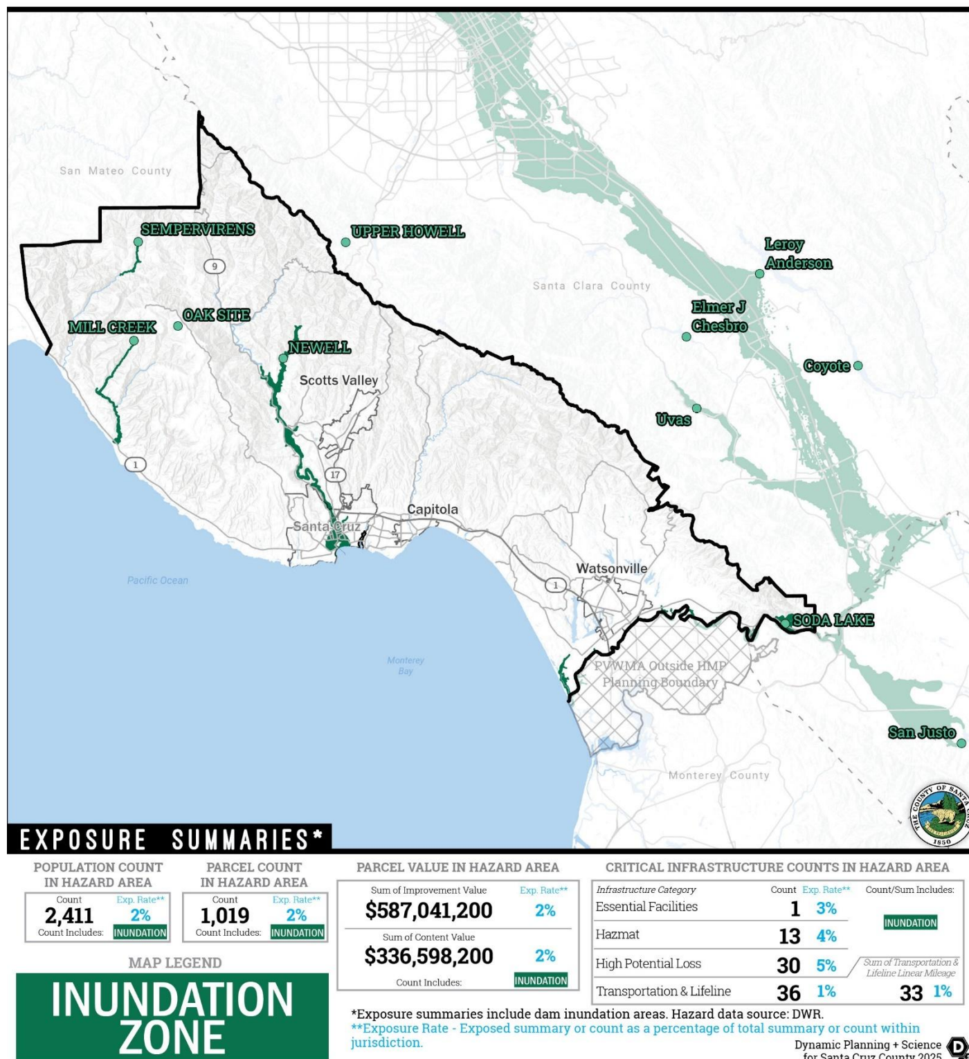
Figure 3-59: Exposure Summary – Santa Cruz County Dam Failure Risk
