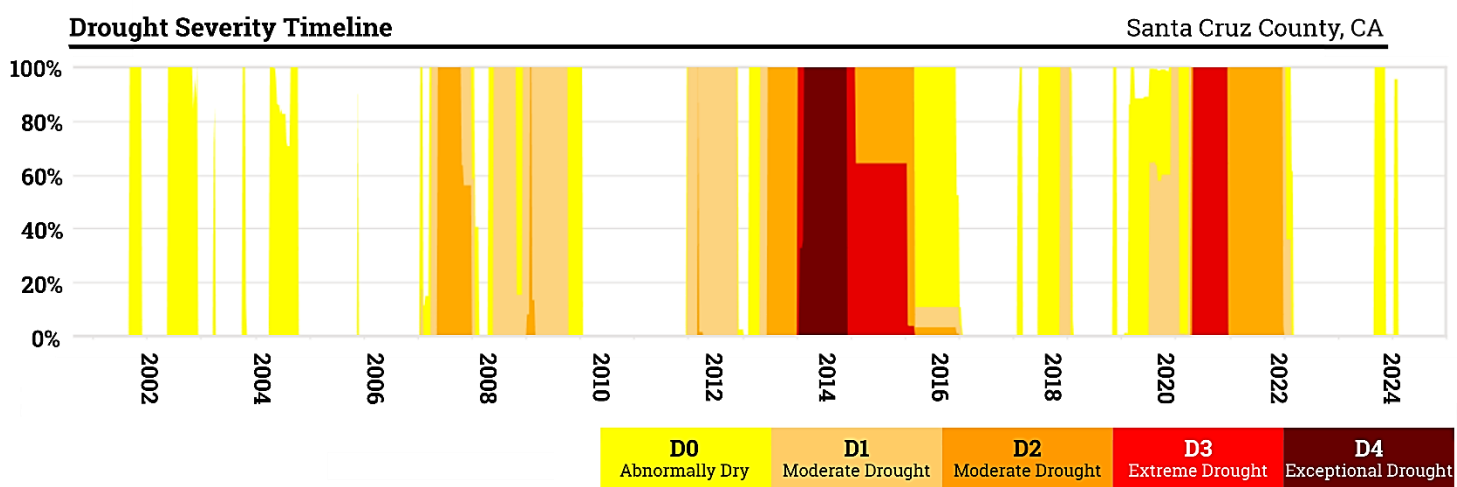
Figure 3-64: County-Wide Drought History and Severity Chart
