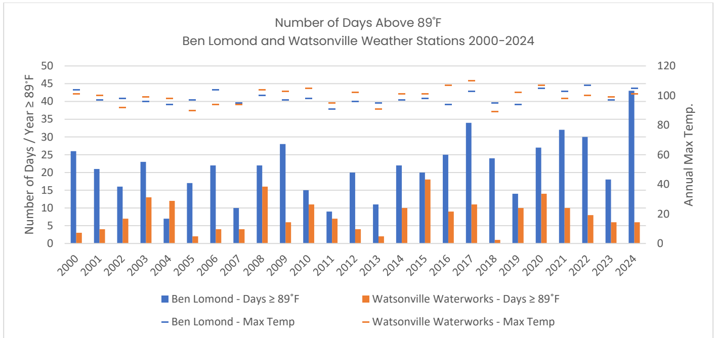
Figure 3-66: Number of Days Above 89°F at Ben Lomond and Watsonville Weather Stations, 2000-2024
